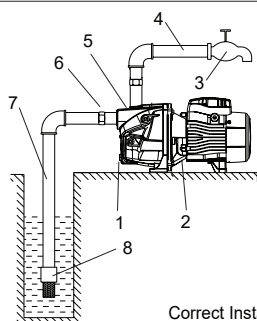
Correct Installation Diagram
